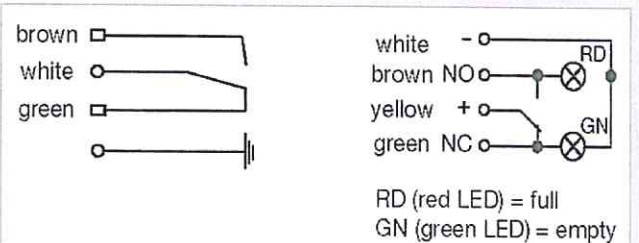
Figure 1: Schematic diagram GK03/GK03-EXI
